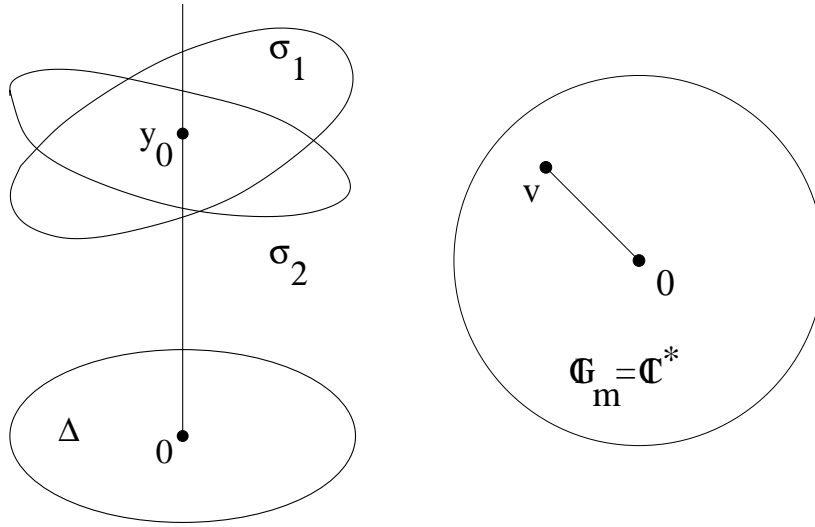
Figure 2.3: Equisingular condition and the path of integration
