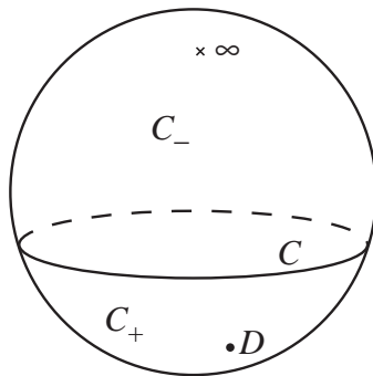
Figure 2.1: Birkhoff Decomposition
