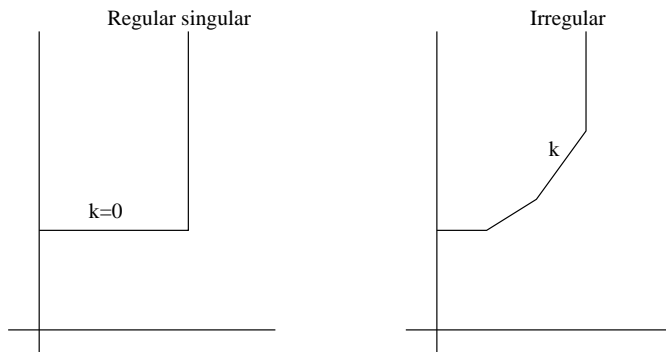
Figure 2.2: Newton polygons
